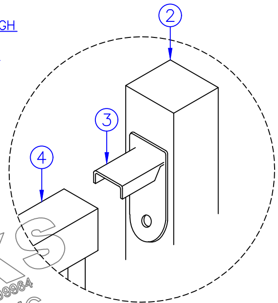
BRACKET ATTACHMENT DETAIL
