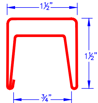
RAIL DETAIL
