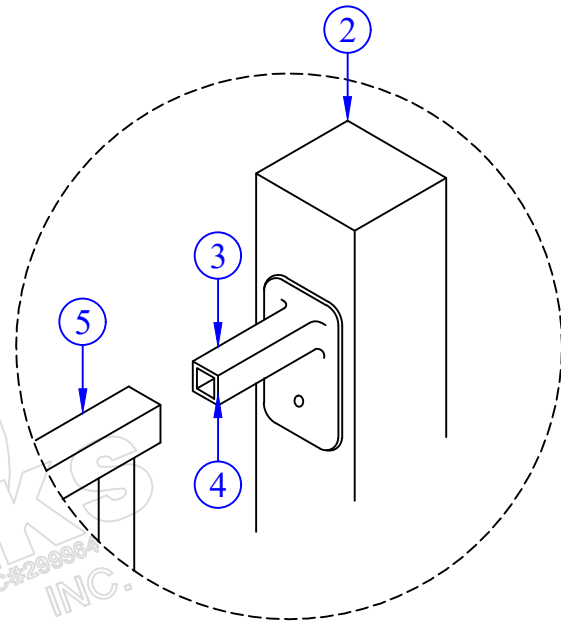
BRACKET ATTACHMENT DETAIL A-A
