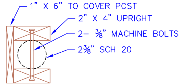
TOP VIEW OF BOLT UP POST
